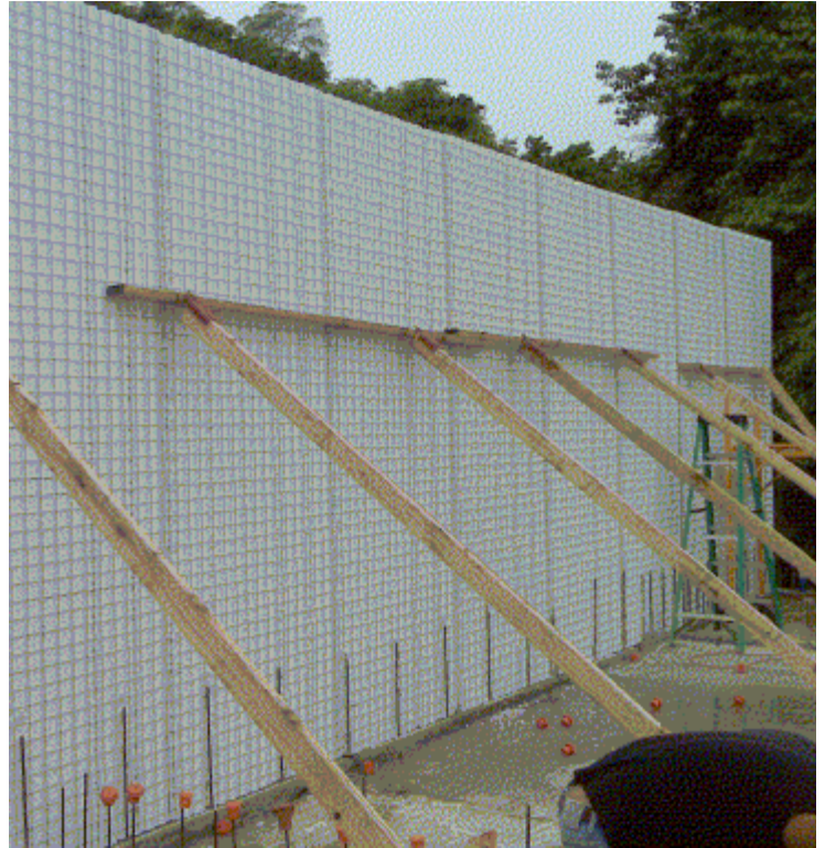
Photo 5: Temporary diagonal wall bracing.
