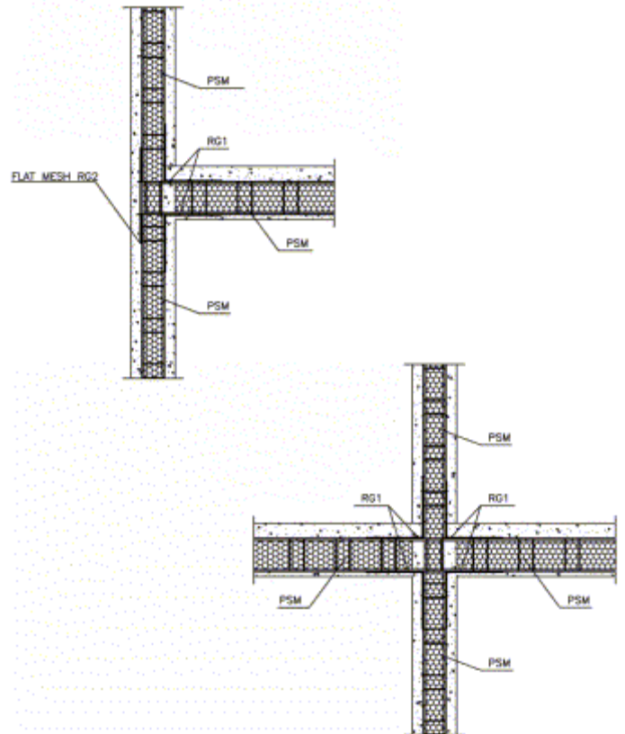
Figure 10: PSM Slab to PSM Wall Connection
