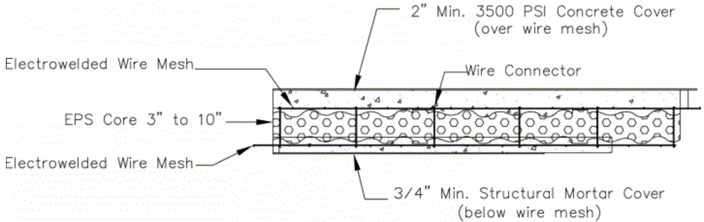
PSM Slab Section
