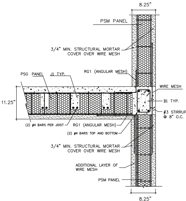
Figure 19b: Example of PSG Floor/Roof attachment where PSG joist is parallel to the wall.
