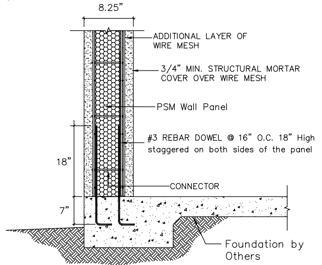
Figure 2: Example of GCT Panel Connection at Exterior Turned Down Slab Footing using rebar anchorage.
