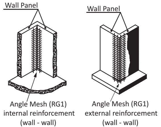
Figure 9: Typical Types of Mesh Used for Reinforcement/Connection
