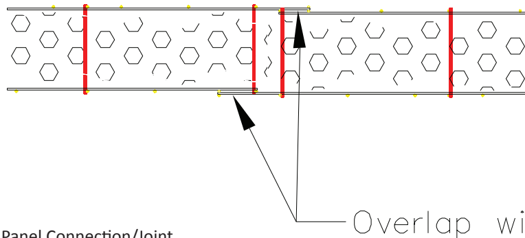
Figure 3: Panel to Panel Connection/Joint
