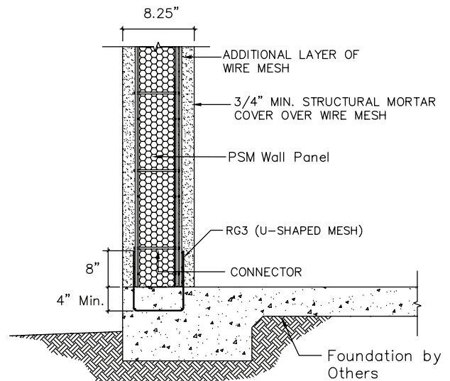
Figure 2a: Example of GCT Panel Connection at Exterior Turned Down Slab Footing using U-shaped wire mesh anchorage.
